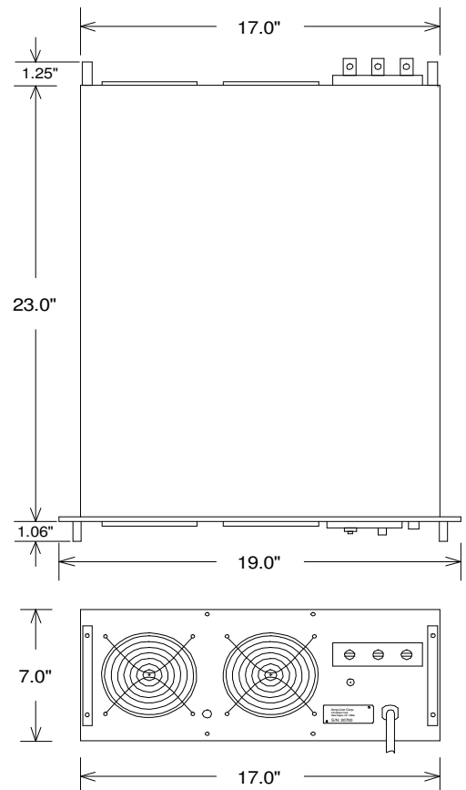
Dimension Drawing
