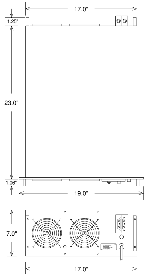
DIMENSION DRAWING
