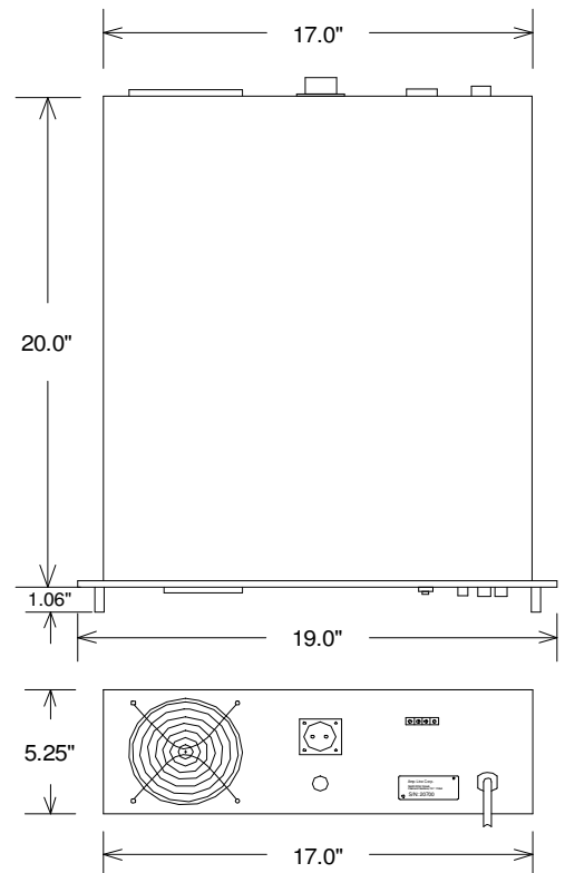
Dimension Drawing
