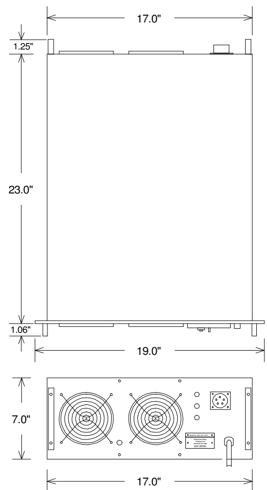
Dimension Drawing
